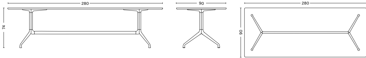
AAT 10 Length 280 cm Width 90 cm Height 74 cm
