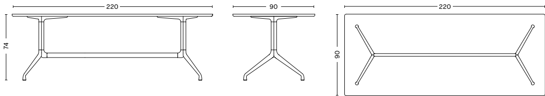
AAT 10 Length 220 cm Width 90 cm Height 74 cm
