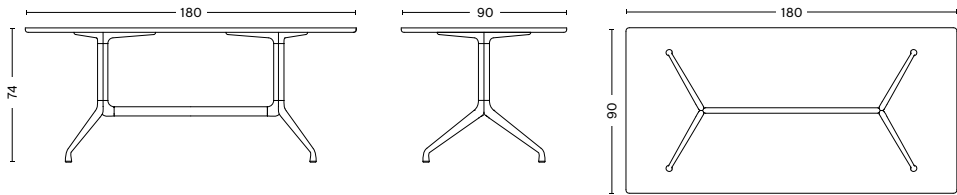
AAT 10 Length 180 cm Width 90 cm Height 74 cm
