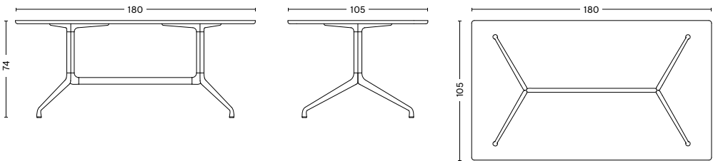
AAT 10 Length 180 cm Width 105 cm Height 74 cm
