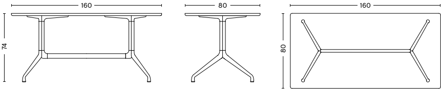
AAT 10 Length 160 cm Width 80 cm Height 74 cm
